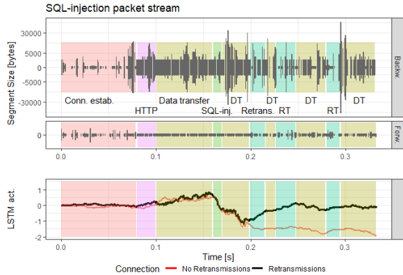
Fig. 3: LSTM-output activation in dependence of connection phases.
